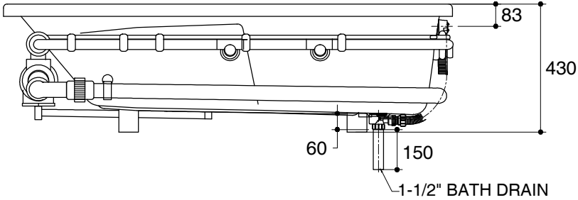
1-1/2" BATH DRAIN
